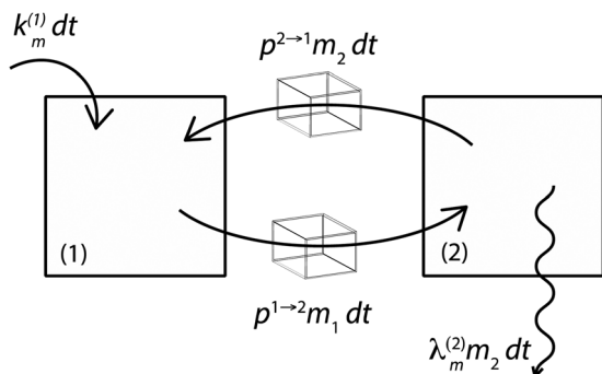
Fig. 3 Illustration of the model for a two-reservoir system. \lambda_m^i is the probability of irreversible loss (excretion) from the i -th reservoir to the surrounding per unit of time, k_m^i is the input flux, p^{i \rightarrow j} is the probability of Zn loss from the i -th reservoir to the j -th reservoir.
