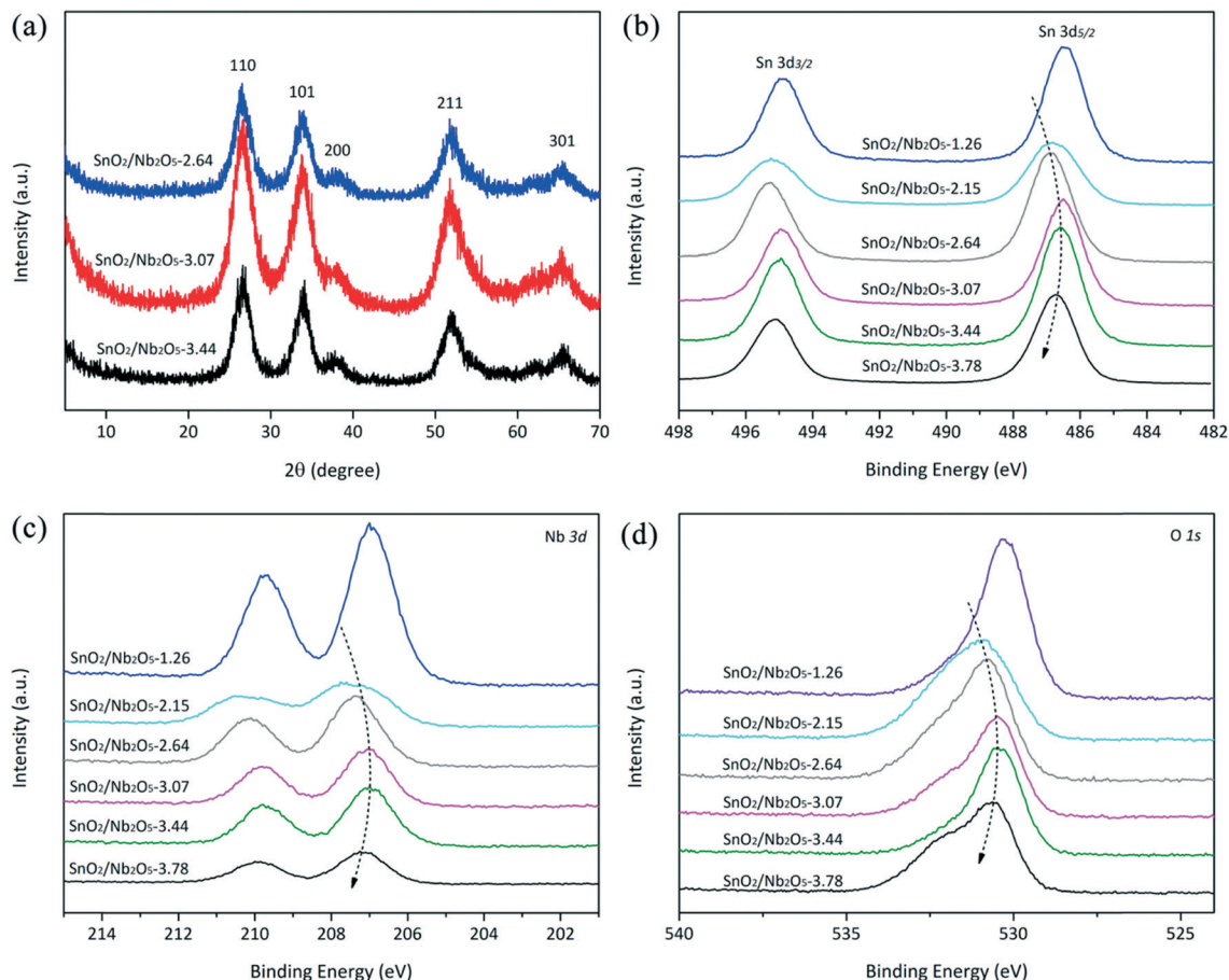
Fig. 2 X-ray diffraction patterns (a) and XPS spectra (b–d) of the \text{SnO}_2/\text{Nb}_2\text{O}_5 samples.
