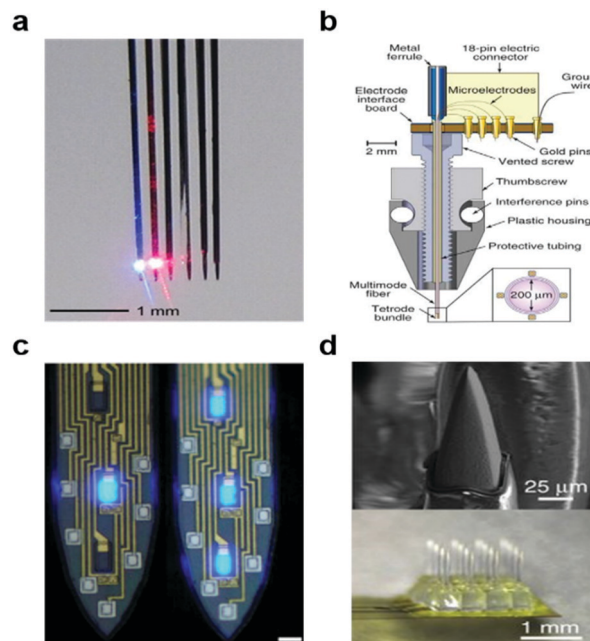
Fig. 9 Optoelectronic neural devices. (a) Multidiod arrays integrated with silicon multielectrodes. Reproduced with permission from ref. 152. Copyright 2012 American Physiological Society. (b) Optetrode with combination of ferrule and Ni/Cr based tetrode bundles. Reproduced with permission from ref. 158. Copyright 2012 Nature Publishing Group. (c) Monolithically integrated \mu LED on silicon neural probe. Reproduced with permission from ref. 164. Copyright 2015 Cell Press. (d) ZnO MOA device for multichannel intracortical neural recording and optical stimulation. Reproduced with permission from ref. 165. Copyright 2015 Nature Publishing Group.
