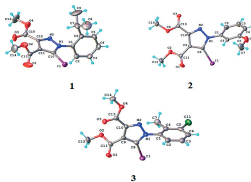
Fig. 3 ORTEP diagrams of the molecules of compounds 1–3 with atom labelling schemes and thermal ellipsoids at the 40% probability level.
