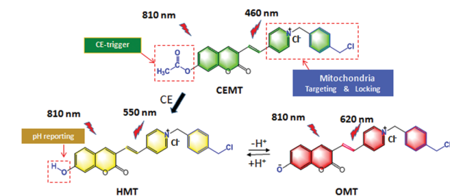
Scheme 1 Design and sensing mechanism of a ratiometric two-photon mitochondria-locked probe CEMT toward carboxylesterase (CE) activity and pH.
