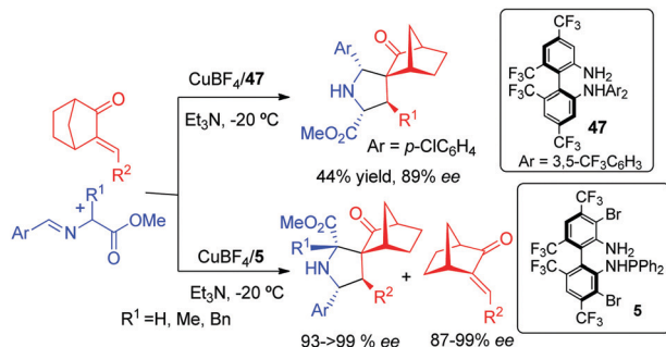
Scheme 29 Cu-Catalyzed 1,3-dipolar cycloaddition of azomethine ylides with alkyldiene norcamphors.
