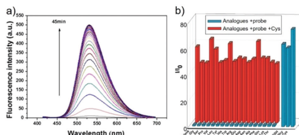
Fig. 98 (a) Time-dependent emission spectra ( \lambda_{\text{ex}} = 400 nm) of probe 61 (10 \mu\text{M} ) upon treatment with Cys (100 equiv.) in DMSO–HEPES (10 mM, pH 7.4, 3:7, v/v) at 37 ^{\circ}\text{C} . Spectra were recorded every min (0–45 min). (b) Blue bars represent probe 61 + analogues; red bars represent probe 61 + Cys in the presence of other analogues (100 \mu\text{M} ). Data were collected at 45 min after addition of each analogue in DMSO–HEPES (10 mM, pH 7.4, 3:7, v/v) at 37 ^{\circ}\text{C} . Copyright 2016 Nature.
