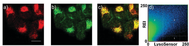
Fig. 16 Confocal fluorescence imaging of living HeLa cells co-stained with probe 12 (5 \mu\text{M} ) and LysoSensor Green (1 \mu\text{M} ) for 1 h. (a) Red emission from probe 12 ; (b) green emission from LysoSensor Green; (c) overlay of (a) and (b); areas of co-localization appeared in yellow; (d) the correlation of LysoSensor Green and probe 12 intensities. Copyright 2015 Elsevier.
