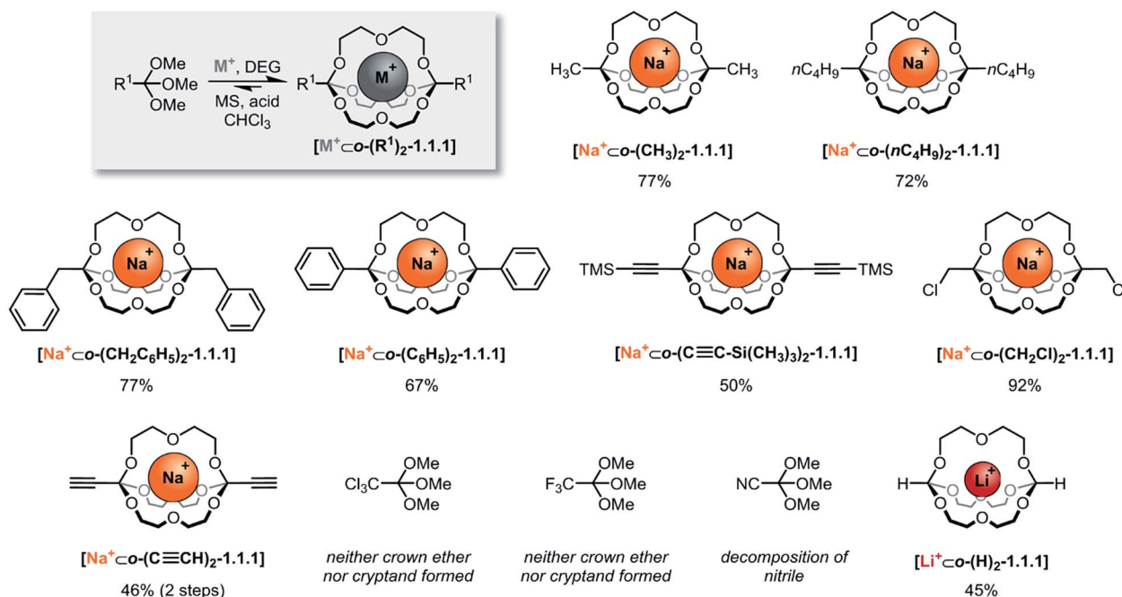
Scheme 2 Scope of self-assembled orthoester cryptands. Reaction conditions: 60 μmol sodium tetrakis[3,5-bis(trifluoromethyl)phenyl]borate (BARF) or LiBARF, 180 μmol diethylene glycol, 120 μmol orthoester, 1.2 μmol TFA ( R^1 = -CH_2Cl : 12 μmol TFA) in CHCl_3 , 7–13 days (for further details, see ESI†). Percent values indicate isolated yields. M^+ : Na^+ ; Li^+ . DEG: diethylene glycol. MS: 5 Å molecular sieves.
