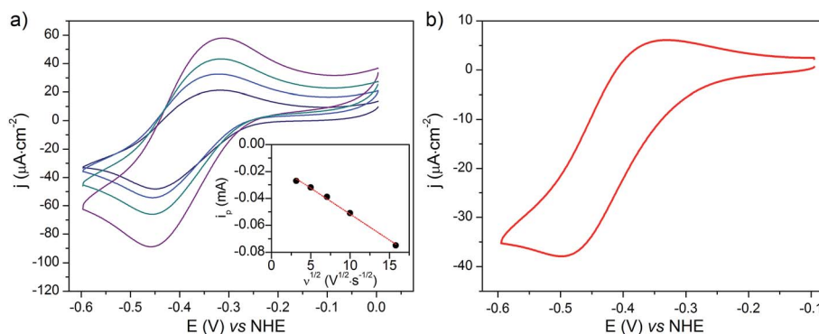
Fig. 8 CVs recorded in a \text{NaCl} 0.1 M aqueous electrolyte at (a) a \text{NiO}|\text{Co}_{\text{C11P}} electrode at scan rates of 10 (navy line), 25 (blue line), 50 (cyan line) and 100 (purple line) \text{mV s}^{-1} with (inset) the dependency of baseline-corrected cathodic peak current on the square root of the scan rate (dots) and its linear fit (dashed lines) and (b) a \text{NiO}|\text{RBG-174}|\text{Co}_{\text{C11P}} electrode at a scan rate of 10 \text{ mV s}^{-1} .
