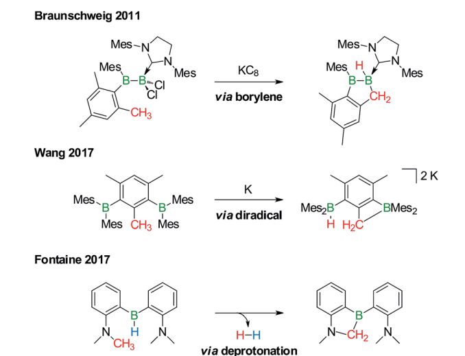
Scheme 2 Selected examples of transition metal-free intramolecular C(sp ^3 )-H activations through borylene (top), diradical (middle), and deprotonation reactions (bottom). Mes = 2,4,6-(H _3\text{C} ) _3\text{C}_6\text{H}_3 .
