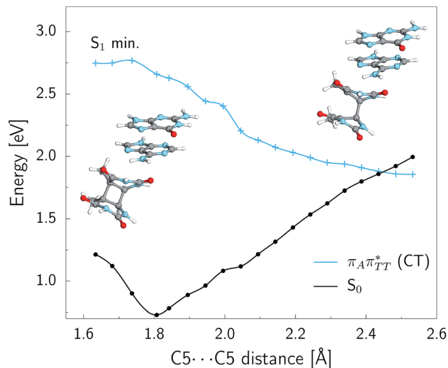
Fig. 6 Potential energy profile presenting the T=T CpD ring opening occurring on the surface of the G^{+}A^{-}T=T^{\cdot-} state. The geometries along the profile were obtained by performing a relaxed scan along the C5...C5 distance using the QM bases /MM setup. The energies presented above were extracted from single-point calculations using the QM DNA /MM setup and the ADC(2)/TZVP method.
