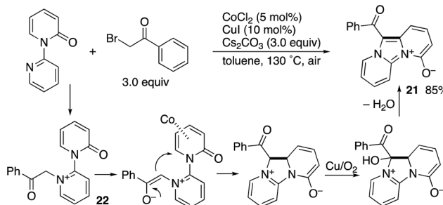
Scheme 24 Rh/Cu-co-catalysed domino alkynylation/oxygenative rearrangement and related Co/Cu aerobic catalysis.
