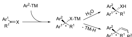
Scheme 2 Conceptual strategies for conjugate or 1,2-arylation reactions.
