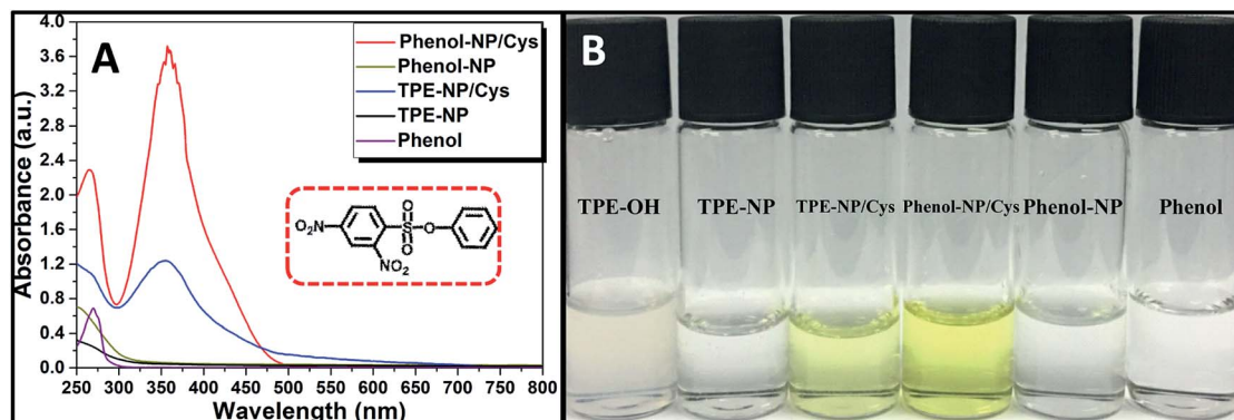
Fig. 5 (A) UV/vis spectra of TPE-NP and phenol-NP solutions (240 \mu\text{M} in PBS/DMSO (v/v = 8/2), pH = 7.4) with and without treatment with Cys and phenol. (B) Photographs of TPE-NP and phenol-NP solutions (240 \mu\text{M} in PBS/DMSO (v/v = 8/2), pH = 7.4) with and without treatment with Cys, TPE-OH and phenol. Inset of part (A) is the structure of phenol-NP.
