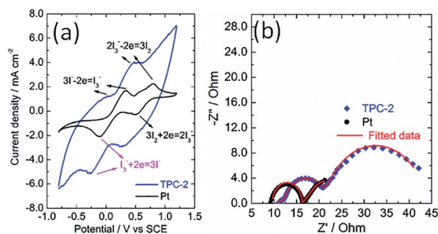
Fig. 5 (a) Cyclic voltammograms for TPC and Pt electrode at a scan rate of 100 \text{ mV s}^{-1} in acetonitrile solution containing 10 mM LiI , 1 mM I_2 , and 0.1 M LiClO_4 with a platinum wire and a SCE electrode used as counter electrode and reference electrode, respectively; (b) Nyquist plots for electrochemical impedance spectra of the symmetrical cells with two identical TPC-2 and Pt electrodes.
