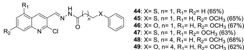
Scheme 9 Condensation of quinolines 16 with hydrazine followed by reaction with substituted-carboxylic acids.
