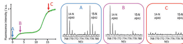
Fig. 14 Mass spectrometric quantification of the relative amount of 14N-A \beta 40 and 15N-A \beta 42 monomers remaining in solution after centrifugation to remove any formed fibrils at time zero (A), after the first sigmoidal transition (B), and after the second sigmoidal transition (C) as observed by ThT fluorescence. At time zero, the solution contained 1.5 \mu M 14N-A \beta 40 monomers and 1.5 \mu M 15N-A \beta 42 monomers. Clearly A \beta 42 is selectively consumed during the first transition, which is thus identified as A \beta 42 fibril formation, and the second transition is identified as A \beta 40 fibril formation. 134
