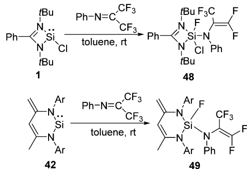
Scheme 17 Activation of the C-F bond in \text{PhC}=\text{N}(\text{CF}_3)_2 by 1 and 42 .
