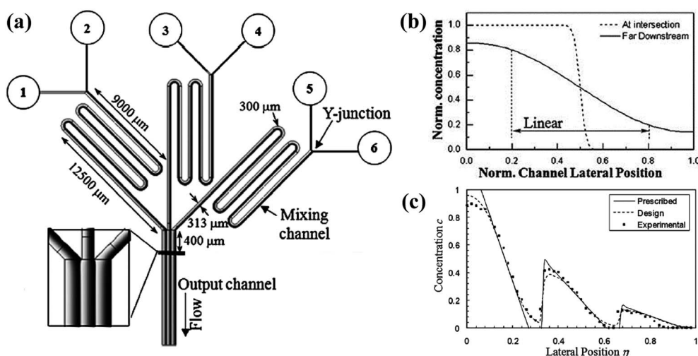
Fig. 4 The schematic diagram of a gradient generator and the obtained gradient profiles. (a) A concentration gradient generator consisted of three Y-shape junctions in parallel. The black line 400 μm downstream of the intersection point shows the position where gradients are measured. (b) Comparisons of the gradient profiles measured at two positions of a Y-shape junction. (c) A sawtooth-shape concentration gradient generated by the device shown in (a). All concentrations in (b) and (c) are normalized. (Reproduced from ref. 100 with permission from the Royal Society of Chemistry).
