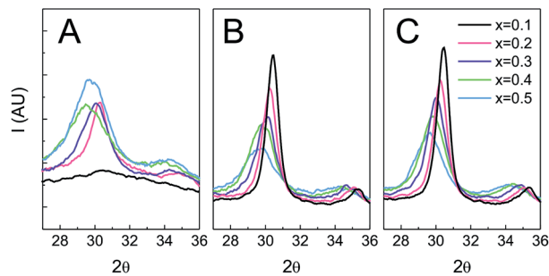
Fig. 8 GIXRD of Zr_{1-x}Ce_xO_2 treated at different temperatures. (A) T = 350 °C; (B) T = 650 °C 30 min; (C) T = 650 °C 3 h.
