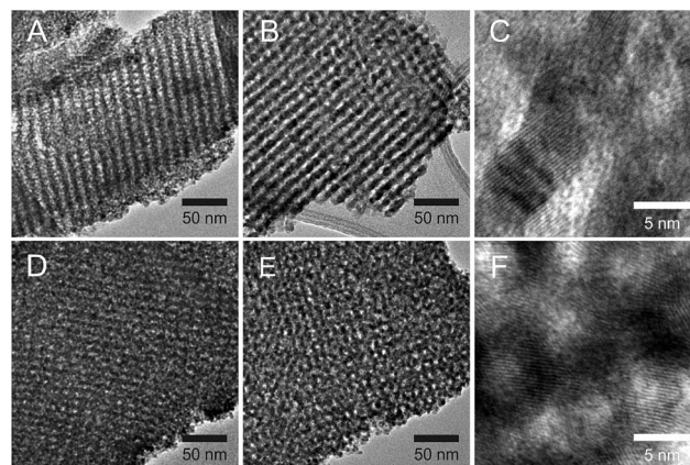
Fig. 9 HR-TEM of Zr_{0.9}Ce_{0.1}O_2 films treated at 350 °C (A) and 550 °C (B and C) and of Zr_{0.5}Ce_{0.5}O_2 films treated at 350 °C (D) and 550 °C (E and F).
