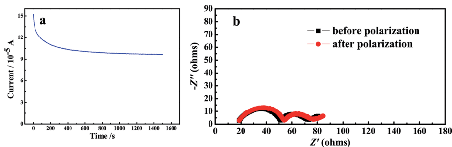
Fig. 7 (a) Chronoamperometry profiles for the GPE at 25 °C in block cells using Li metal as both electrodes with step potential of 10 mV. (b) Nyquist profiles of the cell electrochemical impedance spectroscopy response before and after polarization.
