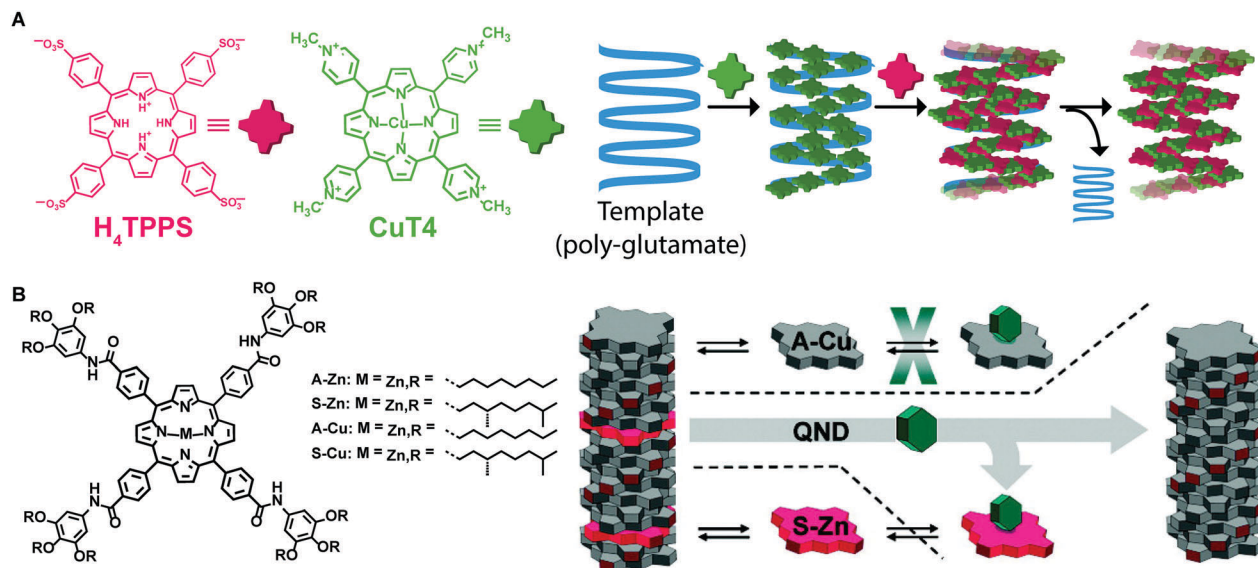
Fig. 11 Template assisted self-assembly. (A) A tetracationic porphyrin ( \text{CuT4} ) is assembled on a polyglutamate template, afterwards, a tetraanionic porphyrin ( \text{H}_4\text{TPPS}_4 ) is assembled in the pre-templated aggregates. Removing the template, the formed assemblies were retained. (B) Chiral porphyrin assemblies were formed via a “sergeant-and-soldier” strategy, removal of the sergeant Zn–porphyrin by axial ligation results in the kinetically trapped assemblies of Cu–porphyrin. Adapted from ref. 48 with permission from the American Chemical Society, copyright 2010.
