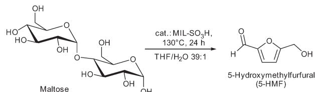
Fig. 23 Conversion of maltose to 5-HMF.
