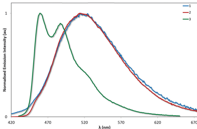
Fig. 8 Normalised emission spectra for complexes 1–3 in deaerated MeCN solution. \lambda_{exc} : 360 nm.
