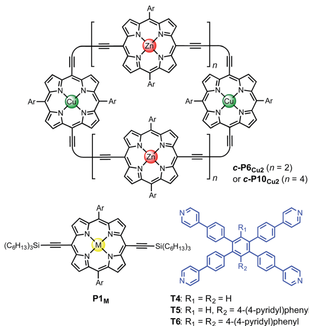
Fig. 1 Chemical structures of the porphyrin nanorings c-P6 Cu2 ( n = 2 ) and c-P10 Cu2 ( n = 4 ), P1 M (where M = \text{Zn}, \text{Cu}, or 2\text{H} ), and the templates T4, T5 and T6. Ar = 3,5-bis( tert -butyl)phenyl.
