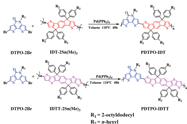
Scheme 1 Synthesis and chemical structures of PDTPPO-IDT and PDTPPO-IDTT .
