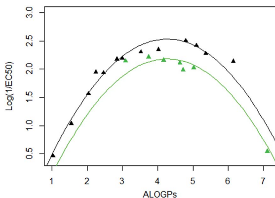
Fig. 6 lmer fit and model for the alkyl R type, OMe ring substituent (coefficients for ALOGPs and ALOGPs-sq are fitted using all data-points). Points coloured by enamine-substituent: black – NH, green – NH-Ph.
