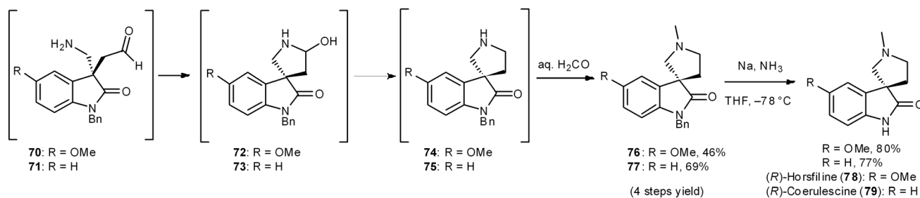
Scheme 7 Three-pot synthesis of (R)-horsifilene and (R)-coerulescine.
