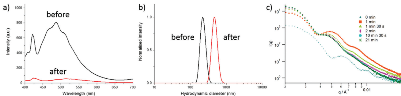
Fig. 2 (a) Fluorescence emission spectra of particles 8 before and after the first CO 2 bubbling, (b) DLS of particles 8 before and after the first CO 2 bubbling, (c) in situ size monitoring of particles 3 by SAXS over 21 min of CO 2 bubbling.
