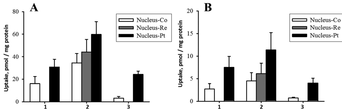
Fig. 6 Nuclear uptake of [\{\text{Co}\}\text{-CN}\text{-}(cis\text{-PtCl}(\text{NH}_3)_2)]^+ ( 1 ), [\{\text{Re}\}\text{-}\{\text{Co}\}\text{-CN}\text{-}(cis\text{-PtCl}(\text{NH}_3)_2)]^+ ( 2 ), and [\{\text{Co}\}\text{-CN}\text{-}(trans\text{-Pt}(\text{Cyt})(\text{NH}_3)_2)]^{2+} ( 3 ) in non-adherent Ehrlich cells (EATC) and adherent Ehrlich Lettre cells (ELA). Uptake was determined as Co, Re, and Pt content in EATC (A) and ELA (B) measured by ICPMS.
