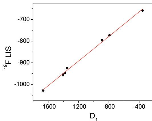
Fig. 4 Graph of D_1 (derived from Bleaney plots of ^1\text{H} shifts of \text{YbL}^{1-7} ) vs. the observed LIS of bound fluoride for \text{YbL}^{1-7} with linear fit in red.
