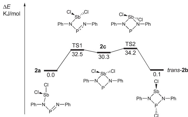
Fig. 5 Potential energy surface of 2M (M = model, terphenyl group substituted by phenyl); the isomerisation process, leading to cis - 2b , was omitted for clarity, see the ESI; ‡ TS = transition state).
