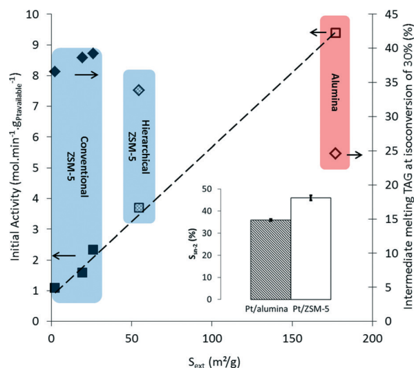
Fig. 5 Influence of S_{\text{ext}} ( S_{\text{total}} in the case of the alumina support) of the various Pt catalysts on the initial activity (calculated as \text{mol}\cdot\text{min}^{-1}(\text{g}_{\text{Pt}} D_{\text{Pt}})^{-1} ) and the hydrogenation selectivity, here expressed as the level of intermediately melting TAGs at 30% conversion ( \text{IV} = 90 ) and the selectivity S_{\text{sn-2}} for the hydrogenation of the fatty acids located at the central sn -2 position, calculated as the conversion on sn -2 / (conversion on sn -2 + conversion on sn -1/3). 100%, at a total conversion of \pm 25 mol% ( \text{IV} = 100 ). All Pt/ZSM-5 catalysts are prepared via competitive ion exchange, whereas Pt/alumina is prepared via incipient wetness impregnation.
