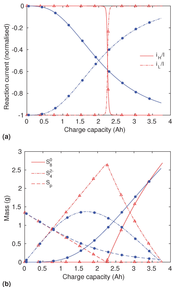
Fig. 4 (a) Simulated reaction currents and (b) species evolution during a 1.7 A (C/2) constant current charge with high saturation concentration S_0^{2-} = 0.005 g, k_p = 100 1/s, (red \Delta ) and low saturation concentration S_0^{2-} = 0.0001 g, k_p = 100 1/s (blue \bullet ). The corresponding voltage is illustrated in Fig. 3(b) with the same symbols. The slower dissolution acts as a bottleneck during charge, triggering an earlier onset of the high plateau reaction and eliminating the boundary between the plateaus. Symbols distinguish between data sets rather than denote computed values.
