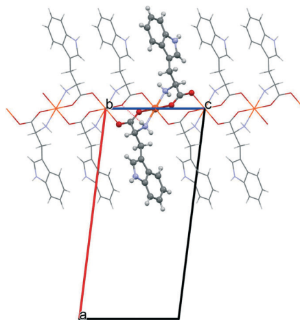
Fig. 2 The packing motif in M( D,L -Try) 2 structures ( 2 ). The central square planar unit is highlighted. The apical connections produce the local distorted octahedron, which gives rise to a bidimensional layer parallel to the bc plane.
