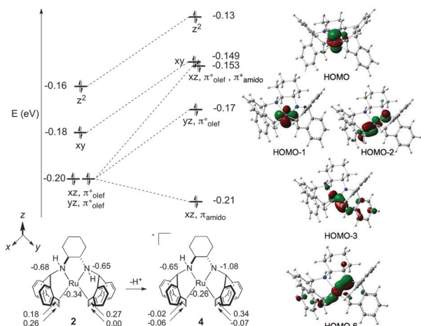
Fig. 2 Top left: Partial orbital energy diagram on going from 2 to 4 with relative orbital energies given in eV. Right: Kohn–Sham orbitals of 4 (isoval = 0.06). Bottom left: Selected APT charges of 2 and 4 given in ESU.
