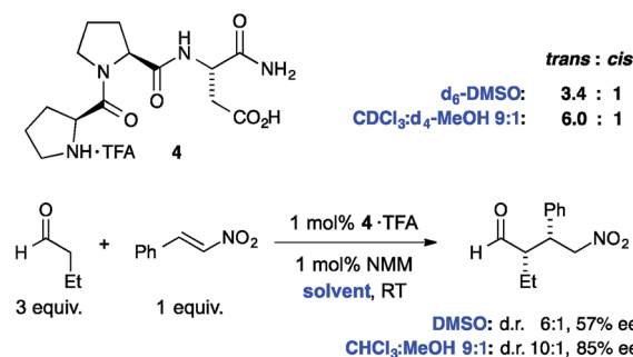
Fig. 7 Trans : cis ratios of the tripeptidic catalyst H-Pro-Pro-Asp-NH 2 ( 4 ) and stereoselectivities of 1,4-addition reactions between butanal and nitrostyrene. a Data taken from ref. 35.
