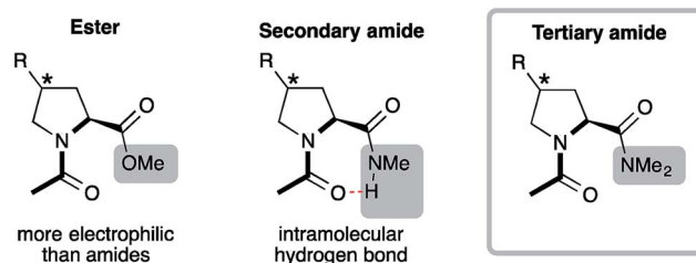
Fig. 2 Acetylated model compounds bearing an ester (Ac–Xaa–OMe), secondary amide (Ac–Xaa–NHMe) and tertiary amide (Ac–Xaa–NMe 2 ).
