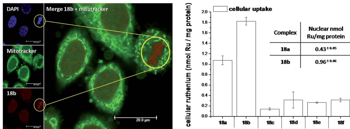
Fig. 16 Left: Confocal microscopy images of HeLa cells treated for 2 h with 100 \mu\text{M} of complex 18b (excitation at 488 nm, emission above 600 nm, bottom left) and stained with DAPI (nuclear staining, top left) and with Mitotracker green (mitochondrial staining, middle left); in the yellow circle a representative example of the different localization of 18b and Mitotracker green is found (picture on the right). Right: Cellular uptake into HeLa cells treated for 4 h with 20 \mu\text{M} solutions of the complexes 18a-f . Results are expressed as the mean \pm error of independent experiments. In the inset: nuclear uptake for complexes 18a and 18b . Reproduced with permission from ref. 53. © 2014 Wiley-VCH Verlag GmbH & Co. KGaA, Weinheim.
