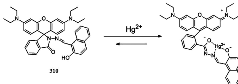
Fig. 272 Chemical structure and proposed mechanism for the fluorescent changes of 310 upon the addition of Hg^{2+} .
