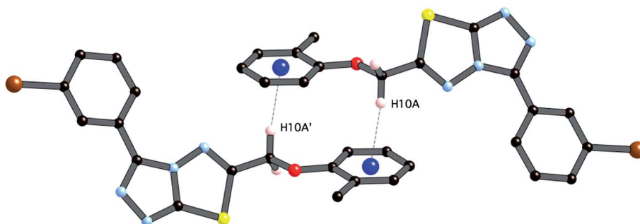
Fig. 5 \text{C-H}\cdots\pi interaction between centrosymmetrically related pairs of 4i , symmetry operator (1 - x, -y, -z) .
