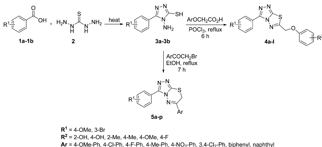
Scheme 1 Synthesis of triazolothiadiazoles ( 4a–l ) and triazolothiadiazines ( 5a–p ).
