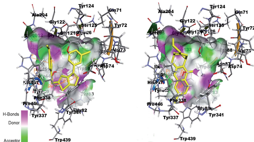
Fig. 13 Binding site interactions of amino acids inside the active pockets of AChE for reference ligand huprine W (right) and the potent compound 4k (left).
