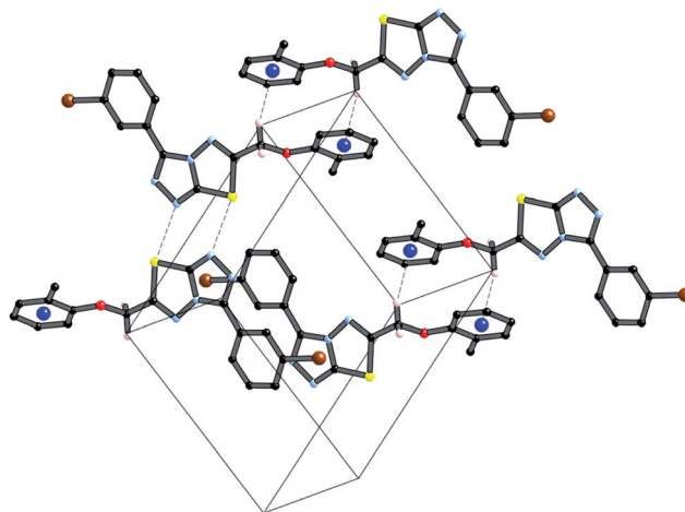
Fig. 6 Partial packing diagram illustrating the \text{N}\cdots\text{S} sigma-hole interaction and the \pi - \pi and \text{C-H}\cdots\pi interactions in crystals of 4i .
