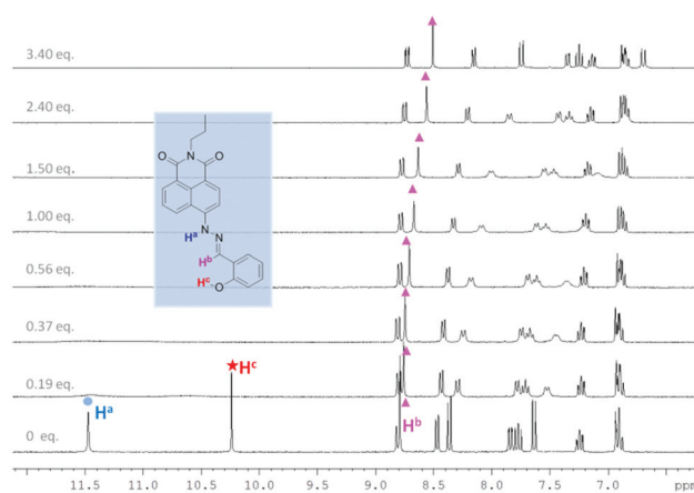
Fig. 7 ^1\text{H} NMR titration of probe 2 with TBAF in \text{DMSO-}d_6 . [\text{2}] = 10.7 \text{ mM} .
