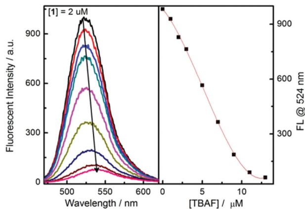
Fig. 5 Fluorescence spectra changes of probe 1 upon addition of TBAF in MeCN. \lambda_{\text{ex}} = 450 \text{ nm} , [\text{1}] = 2 \mu\text{M} .
