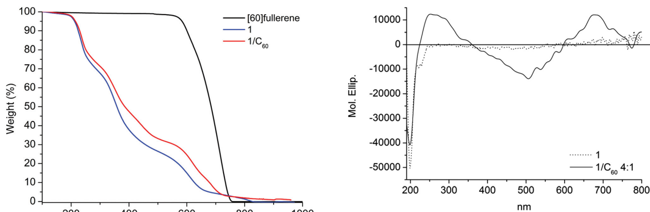
Fig. 4 CD spectra of aqueous solutions of peptide 1 (dotted line) and 1/C 60 obtained by HSV (solid line).
