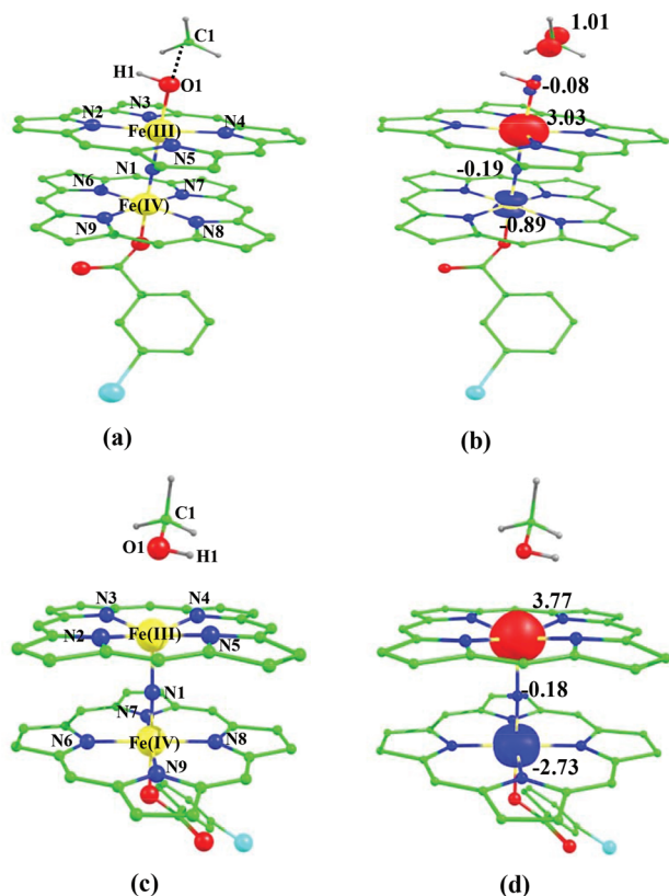
Fig. 8 B3LYP-D2 optimized structure of (a) {}^4\text{ts}2_{(\text{hs}, \text{hs})} state. Spin density plot computed for (b) {}^4\text{ts}2_{(\text{hs}, \text{hs})} state. Optimized structure of (c) {}^2P_{(\text{hs}, \text{hs})} state and (d) its corresponding spin density plot. The bond parameters computed for the spin states are given below with the following notations {}^4\text{ts}2_{(\text{hs}, \text{hs})} ( {}^4\text{ts}2_{(\text{ls}, \text{ls})} ) [ {}^8\text{ts}2_{(\text{ls}, \text{ls})} ]. Fe(III)–N1 = 1.719 (1.886) [1.952], Fe(III)–N2 = 2.073 (2.061) [2.064], Fe(III)–N3 = 2.075 (2.105) [2.098], Fe(III)–N4 = 2.083 (2.052) [2.061], Fe(III)–N5 = 2.097 (2.110) [2.099], Fe(IV)–N1 = 1.649 (1.742) [1.880], Fe(IV)–N6 = 2.028 (2.021) [2.029], Fe(IV)–N7 = 2.016 (2.024) [2.009], Fe(IV)–N8 = 2.011 (2.012) [2.019], Fe(IV)–N9 = 2.015 (2.010) [1.996], Fe(III)–O1 = 1.901 (1.861) [1.856], O1–H1 = 0.982 (0.983) [0.983], O1–C1 = 2.488 (2.415) [2.441], \angle\text{Fe(III)}-\text{N1}-\text{Fe(IV)} = 179.5 (178.2) [174.9], \angle\text{Fe(III)}-\text{O1}-\text{H1} = 108.0 (111.4) [111.6], \angle\text{Fe(III)}-\text{O1}-\text{C1} = 128.3 (135.8) [135.4]. For species P , {}^2P_{(\text{hs}, \text{hs})} ( {}^6P_{(\text{ls}, \text{ls})} ) [ {}^{10}P_{(\text{hs}, \text{hs})} ]. Fe(III)–N1 = 1.773 (1.743) [1.951], Fe(III)–N2 = 2.108 (2.027) [2.090], Fe(III)–N3 = 2.121 (2.029) [2.102], Fe(III)–N4 = 2.085 (2.010) [2.069], Fe(III)–N5 = 2.082 (2.013) [2.079], Fe(IV)–N1 = 1.652 (2.089) [1.855], Fe(IV)–N6 = 2.078 (2.026) [2.088], Fe(IV)–N7 = 2.095 (2.032) [2.088], Fe(IV)–N8 = 2.075 (2.015) [2.086], Fe(IV)–N9 = 2.073 (2.022) [2.069], Fe(IV)–O1 = 2.468 (2.183) [2.285], O1–H1 = 0.981 (0.983) [0.979], O1–C1 = 1.457 (0.979) [1.462], \angle\text{Fe(III)}-\text{N1}-\text{Fe(IV)} = 178.6 (179.7) [179.4], \angle\text{Fe(III)}-\text{O1}-\text{H1} = 85.6 (98.1) [96.9], \angle\text{Fe(III)}-\text{O1}-\text{C1} = 116.4 (116.7) [116.3]. All the distances are given in Å and angles in °.
