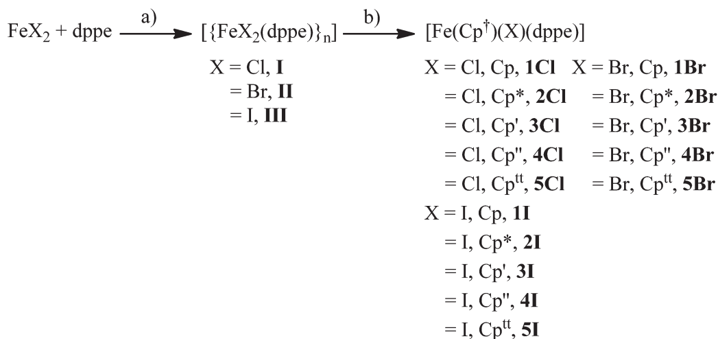
Scheme 1 Synthesis of I , II , III , 1Cl–5Cl , 1Br–5Br , 1I–5I . Reagents and conditions: (a) THF, \Delta ; (b) \text{LiCp}/\text{NaCp}/\text{KCp}^+ , toluene, -78^\circ\text{C} , -\text{LiCl}/\text{KCl}/\text{NaI}/\text{KCl}/\text{KBr}/\text{KI} .
