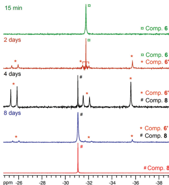
Fig. 3 ^{31}\text{P}\{^1\text{H}\} NMR (162 MHz, \text{CD}_2\text{Cl}_2 , RT) monitoring of the conversion of heteroleptic species 6 to homoleptic 8 via the formation of species 6' . Conditions: [\text{6}]_0 = 10 \text{ mM} , \text{CD}_2\text{Cl}_2 , room temperature. For comparison, the ^{31}\text{P}\{^1\text{H}\} NMR spectrum of analytically pure compound 8 (bottom spectrum) prepared and isolated from the reaction of \text{ZnEt}_2 and 2 equiv. of ligand 2-H is shown.
