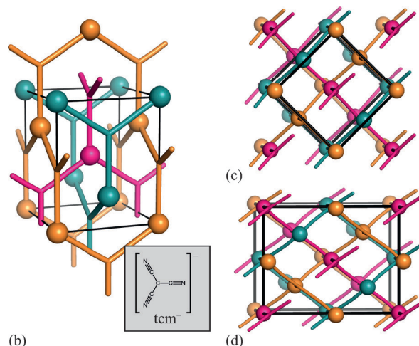
Fig. 3 (a) Representation of the crystal structure of \beta\text{-Cu}(\text{tcm}) , viewed with the tetragonal c axis oriented vertically. Thermal ellipsoids are represented at 50% probability. (b) Topological representation of the same framework, where Cu atoms are shown as large spheres, tcm moieties in stick representation, and the unit cell in black. The three mutually-interpenetrating (10,3)- b frameworks are coloured differently. The inset shows the chemical structure of the tricyanomethanide anion. (c) The same framework, viewed slightly away from c , illustrating its square wine-rack geometry with \theta = 90^\circ . (d) The low-temperature \alpha\text{-Cu}(\text{tcm}) phase—shown here in terms of the structural model determined using powder X-ray diffraction data collected at 20 K—has the same network connectivity, but the loss of tetragonal symmetry allows \theta to deviate from 90^\circ . The Fdd2 unit cell, shown here in black, has twice the volume of the I4_1md cell of \beta\text{-Cu}(\text{tcm}) .
