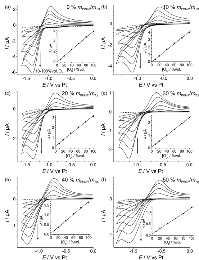
Fig. 4 Cyclic voltammetry of the O_2/O_2^{\bullet-} redox couple at 10, 20, 40, 60, 80, 100% vol. O_2 in the flow (500 sccm), for PMMA- [C_2\text{mim}][\text{NTf}_2] mixtures at 0–50% m_{\text{PMMA}}/m_{\text{Tot}} , carried out with a scan rate of 100\text{ mV s}^{-1} vs. Pt pseudo-RE. The dotted lines are the CVs in the absence of oxygen. The insets are corresponding plots of O_2 reduction peak current vs. %vol. O_2 in the flow, and the line of best-fit.
