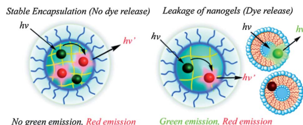
Scheme 6 Mechanism of the FRET experiment in comparing the stability of nanogels with or without a reducing agent. 74
