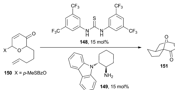
Scheme 20 Oxidopyrylium cycloaddition catalysed by 148 and 149 .
