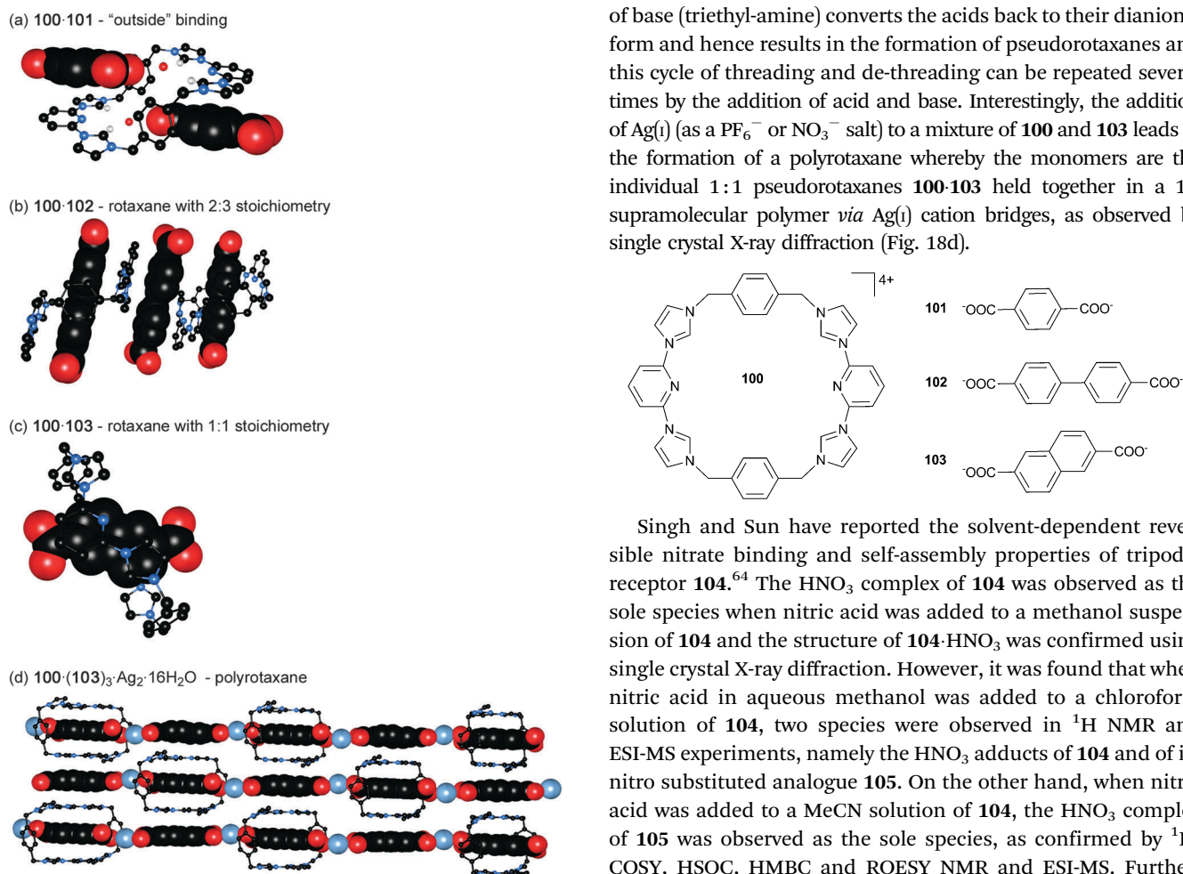
Fig. 18 Crystal structures of Sessler’s tetracationic macrocycle with various dianions. Hydrogen atoms, solvent molecules and counterions have been omitted for clarity; the dianions are shown in spacefill with the macrocycle in ball-and-stick. (a) [\mathbf{100}\cdot\mathbf{101}]^{2+} showing that the dianion is bound outside the macrocycle (no threading); (b) [\mathbf{100}\cdot\mathbf{102}]^{2+} showing rotaxane formation with 2:3 stoichiometry; (c) [\mathbf{100}\cdot\mathbf{103}]^{2+} showing rotaxane formation with 1:1 stoichiometry; (d) \mathbf{100}\cdot(\mathbf{103})_3\cdot\text{Ag}_2\cdot 16\text{H}_2\text{O} showing polyrotaxane formation upon the addition of \text{Ag}(\text{I}) .
