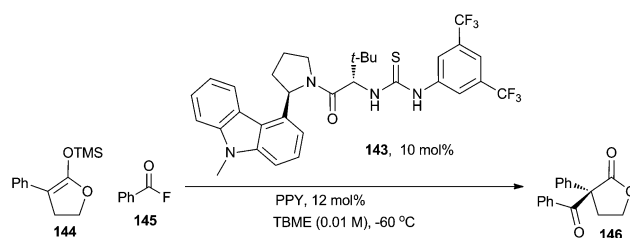
Scheme 18 Conversion of 144 into 146 catalysed by thiourea 143 and PPY.
